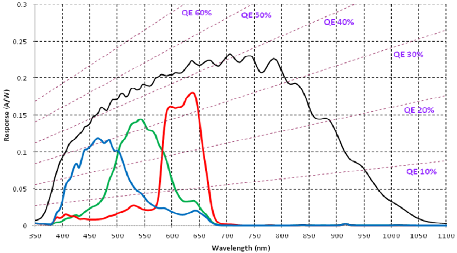
Color and Spectral Response Curve
